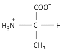
Alanina
